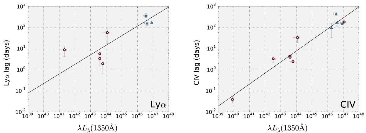
FIGURE 3 | Ly \alpha ( Left ) and CIV ( Right ) radius–luminosity relations. Blue triangles correspond to results from our high- z , high-luminosity sample, while red circles are taken from the literature. These are NGC3783, NGC5548, NGC7469, F9, and 3C390.3 for the Ly \alpha relation, and NGC4395, NGC5548, NGC3783, NGC7469, and 3C390.3 for the CIV relation (Peterson et al., 2005, 2006; De Rosa et al., 2015; Lira et al., submitted). Taken from Lira et al. (submitted), ©AAS.
