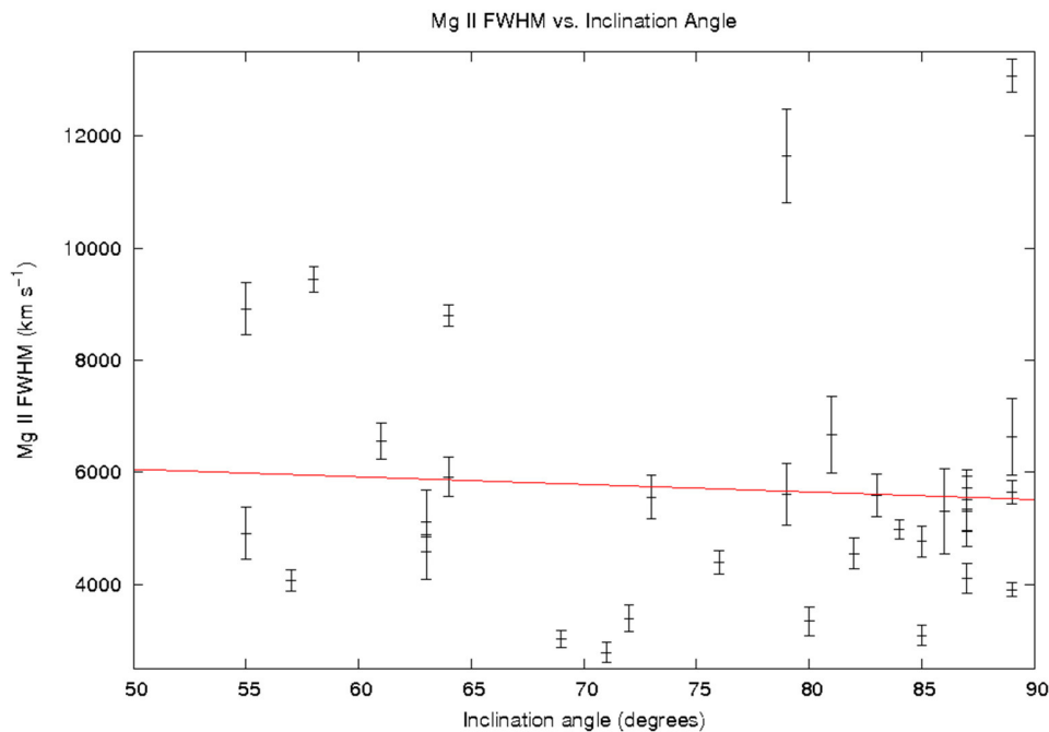
FIGURE 2 | Quasar Mg II FWHM plotted against inclination angle, with vertical bars at each point indicating FWHM 1\sigma error range for each object. A best-fitting trend line (red) shows a small negative gradient, however a Pearson test indicates no correlation.
