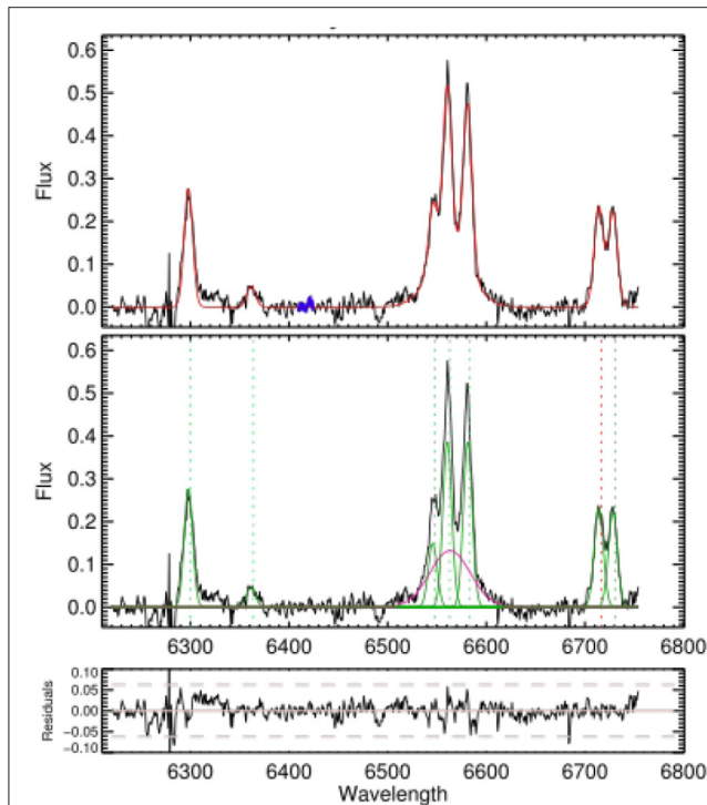
FIGURE 6 | Top: Stellar population subtracted spectrum of NGC 3718 (black), together with the final model with single Gaussian components for the narrow lines and an additional very broad component for H \alpha . Middle: Narrow line fitting in green and very broad H \alpha in magenta. Bottom: Residual spectrum.
