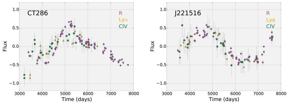
FIGURE 2 | Shifted and normalized continuum and emission line light curves for CT286 ( Left ) and J221516 ( Right ). The time axis is expressed in Julian Dates - 2,450,000 days. R-band continuum, Ly \alpha , and CIV light curves are presented using circles, triangles, and squares, respectively.
