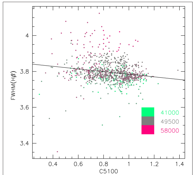
FIGURE 6 | Anti-correlation between FWHM of H\beta and continuum specific flux at 5100 Å. The line shows an unweighted least squares fit. Colors of data points are coded from green to magenta according to Julian date, from 2441000 to 2458000.
