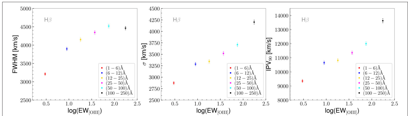
FIGURE 1 | Full Width Half Maximum, Inter-Percentile Velocity width and dispersion \sigma as a function of the EW_{[OIII]} for the H \beta line. All these quantities, describing the rotational velocity of the gas orbiting around the central SMBH, increase moving from low to high EW_{[OIII]} as expected if the BLR is disc-shaped and we are moving from face-on to edge-on positions.
