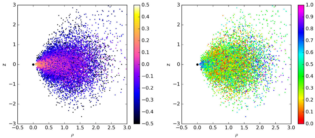
FIGURE 3 | Distribution of clouds in the torus. All particles are gathered in the meridional plane ( \rho, z ), where \rho = \sqrt{x^2 + y^2} . Left panel: colors mark the deviations of the cloud velocity in the torus ( V ) from a keplerian velocity for the case of a disk ( V_k ): ( V/V_k - 1 ). Right panel: colors mark the values of the eccentricity of the cloud orbits.
