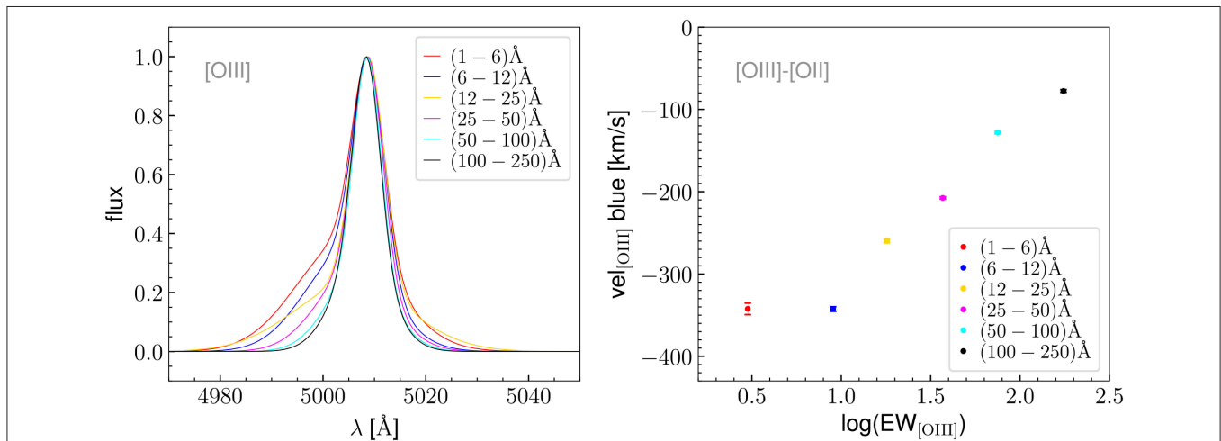
FIGURE 2 | Left: [OIII] 5007 Å line profile as a function of EW_{[OIII]} . The blue component of the line decreases moving from low to high EW_{[OIII]} . Right: velocity shift of the blue component of the [OIII] line with respect to the velocity of the [OII] \lambda 3727 line, accounting for the systemic velocity of the host galaxy. The shift is decreasing (in modulus) when moving from low to high EW_{[OIII]} . Both the trends are expected if we are moving from face-on to edge-on positions, where the outflow velocity component of the gas is not intercepted anymore by the line of sight.
