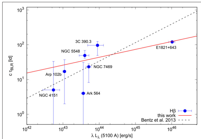
FIGURE 4 | The radius of the broad H\beta line emitting-region vs. the continuum luminosity at 5100 Å. The dashed line gives the BLR radius-luminosity scaling relation from Bentz et al. (2013) with R_{\text{BLR}} \propto L^{0.533} , whereas the solid line is the fit through seven objects from this study, with R_{\text{BLR}} \propto L^{0.226} . We note that the fit is strongly influenced from the one point, the luminous quasar E1821+643, and without that point the relation is consistent with the Bentz et al. (2013) result.
