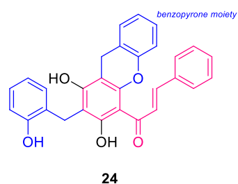
FIGURE 4 Chemical structures of chalcones isolated from Annonaceae (1–25).
