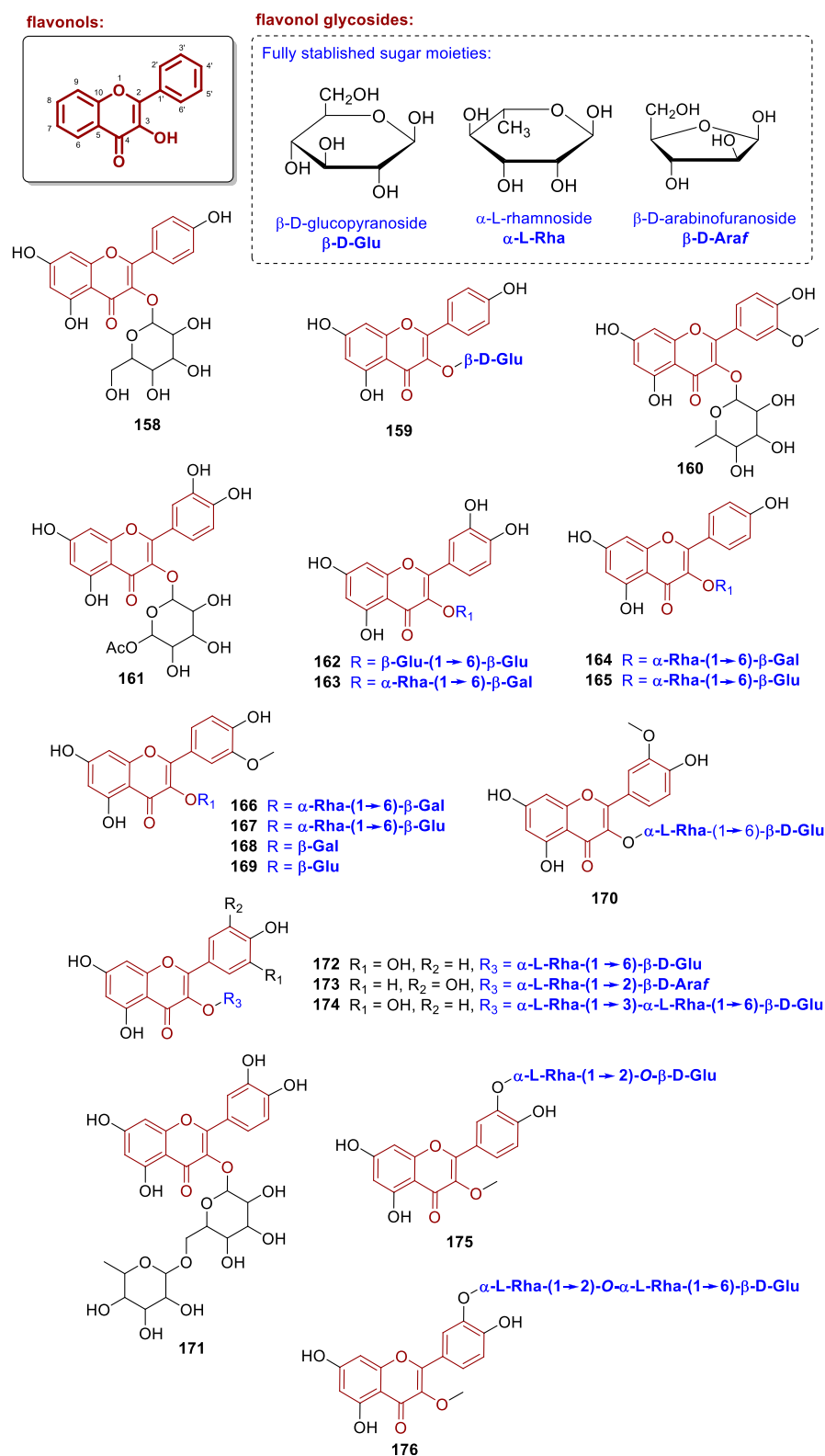
FIGURE 11 Chemical structures of flavonol glycosides isolated from Annonaceae (158–176).
