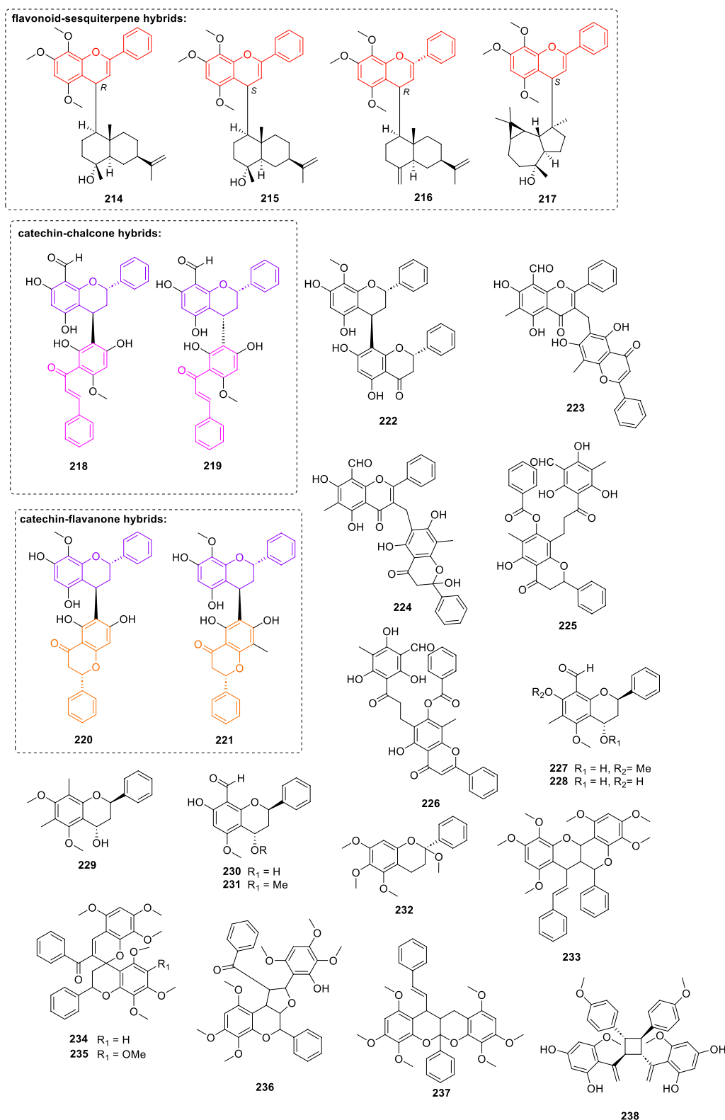
FIGURE 15 Chemical structures of miscellaneous compounds isolated from Annonaceae ( 214–238 ).
