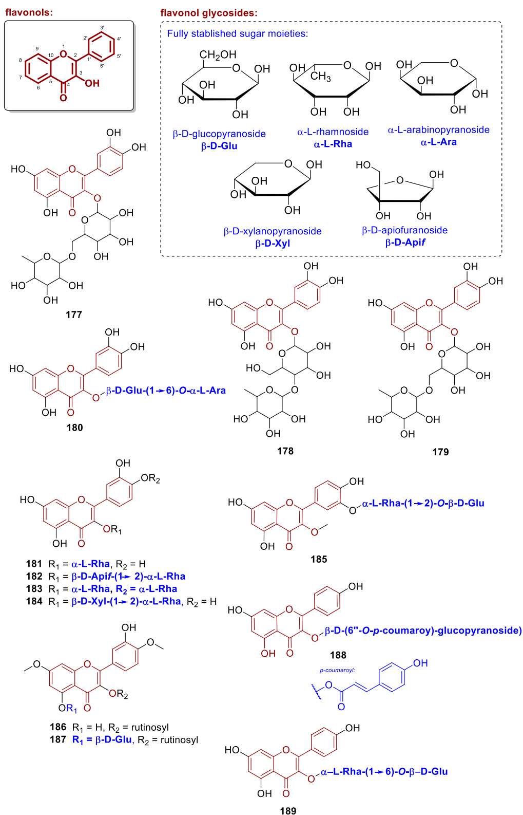
FIGURE 12 Chemical structures of flavonol glycosides isolated from Annonaceae (177–189).
