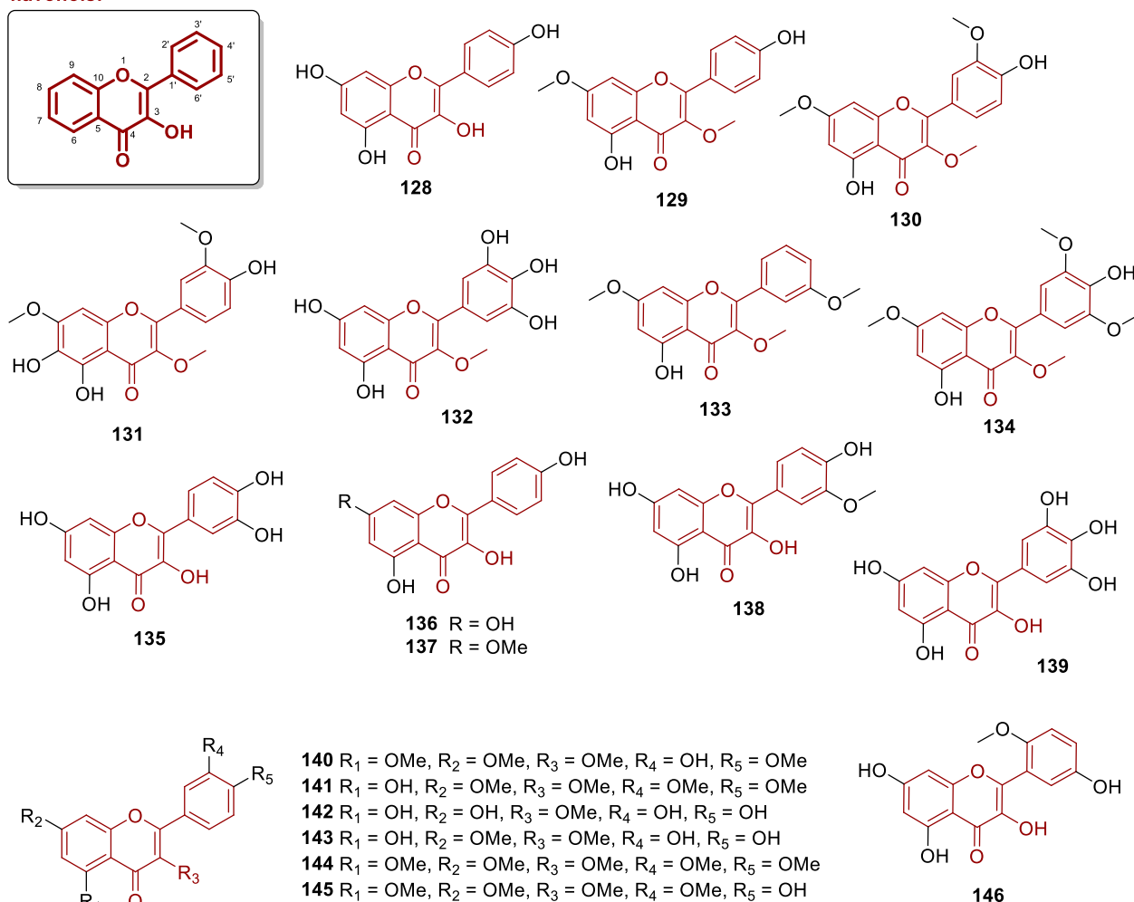
FIGURE 9 Chemical structures of flavonol aglycones isolated from Annonaceae (128–146).
