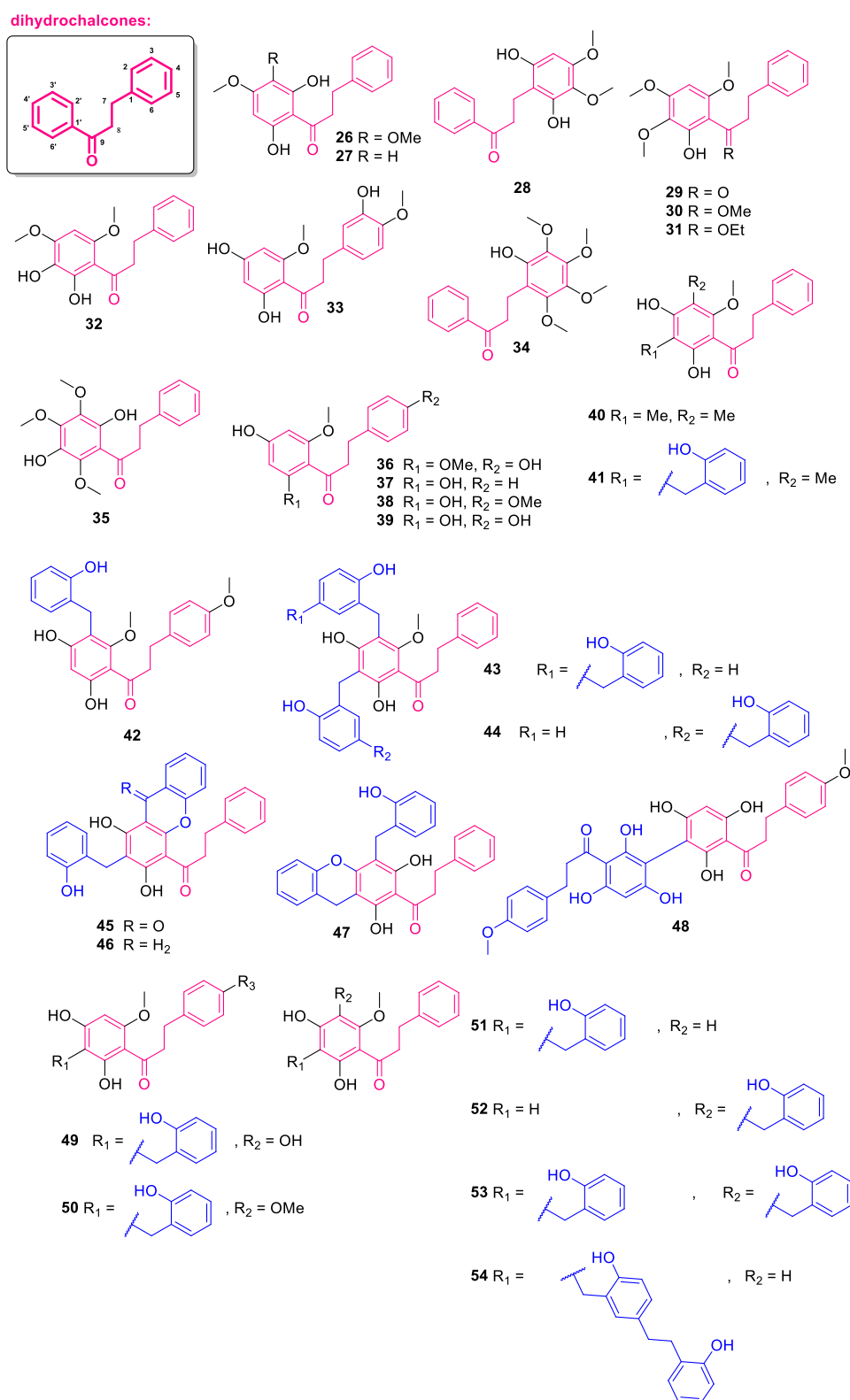
FIGURE 5 Chemical structures of dihydrochalcones isolated from Annonaceae (26–54).
