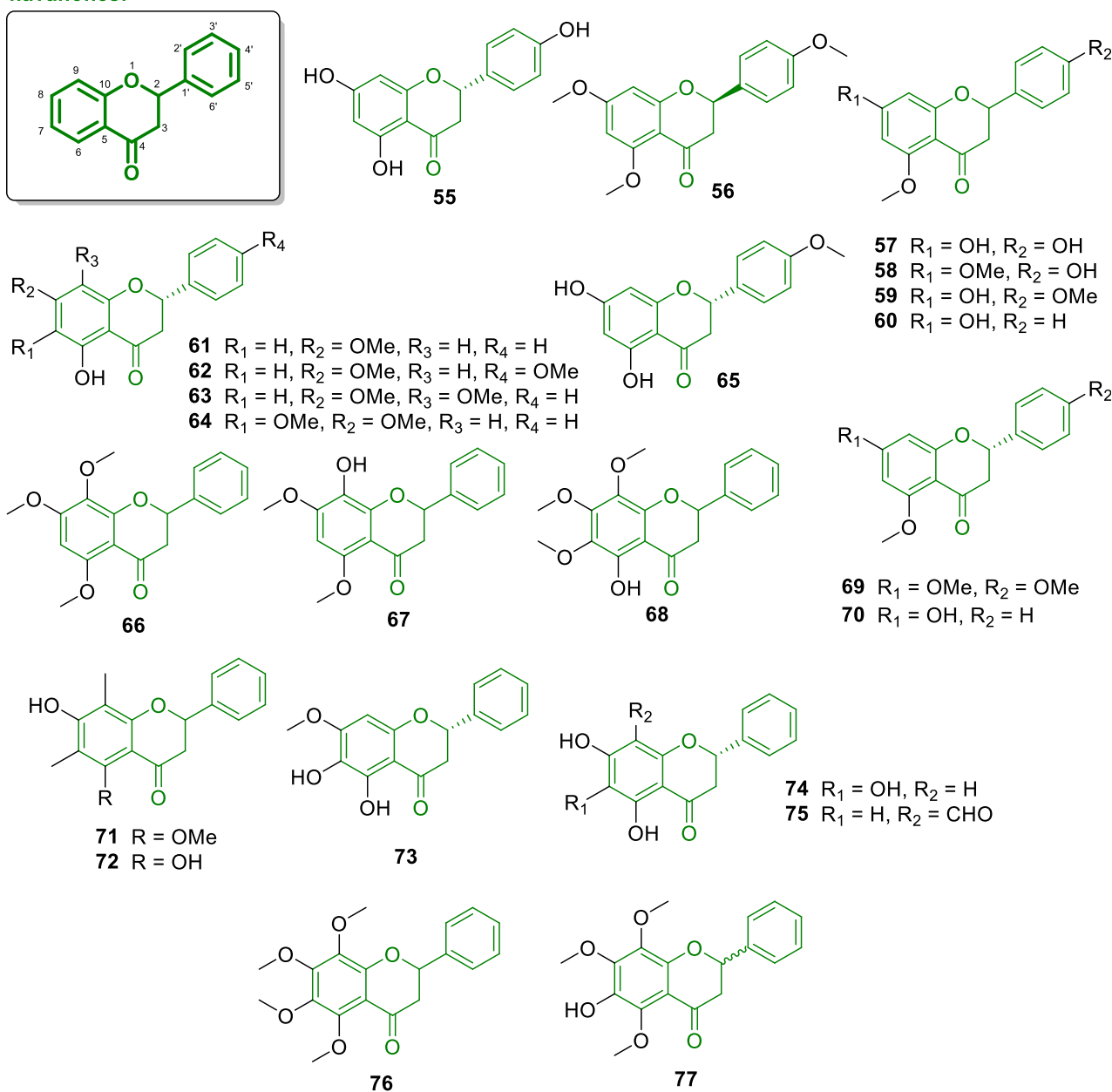
FIGURE 6 Chemical structures of flavanones isolated from Annonaceae (55–77).
