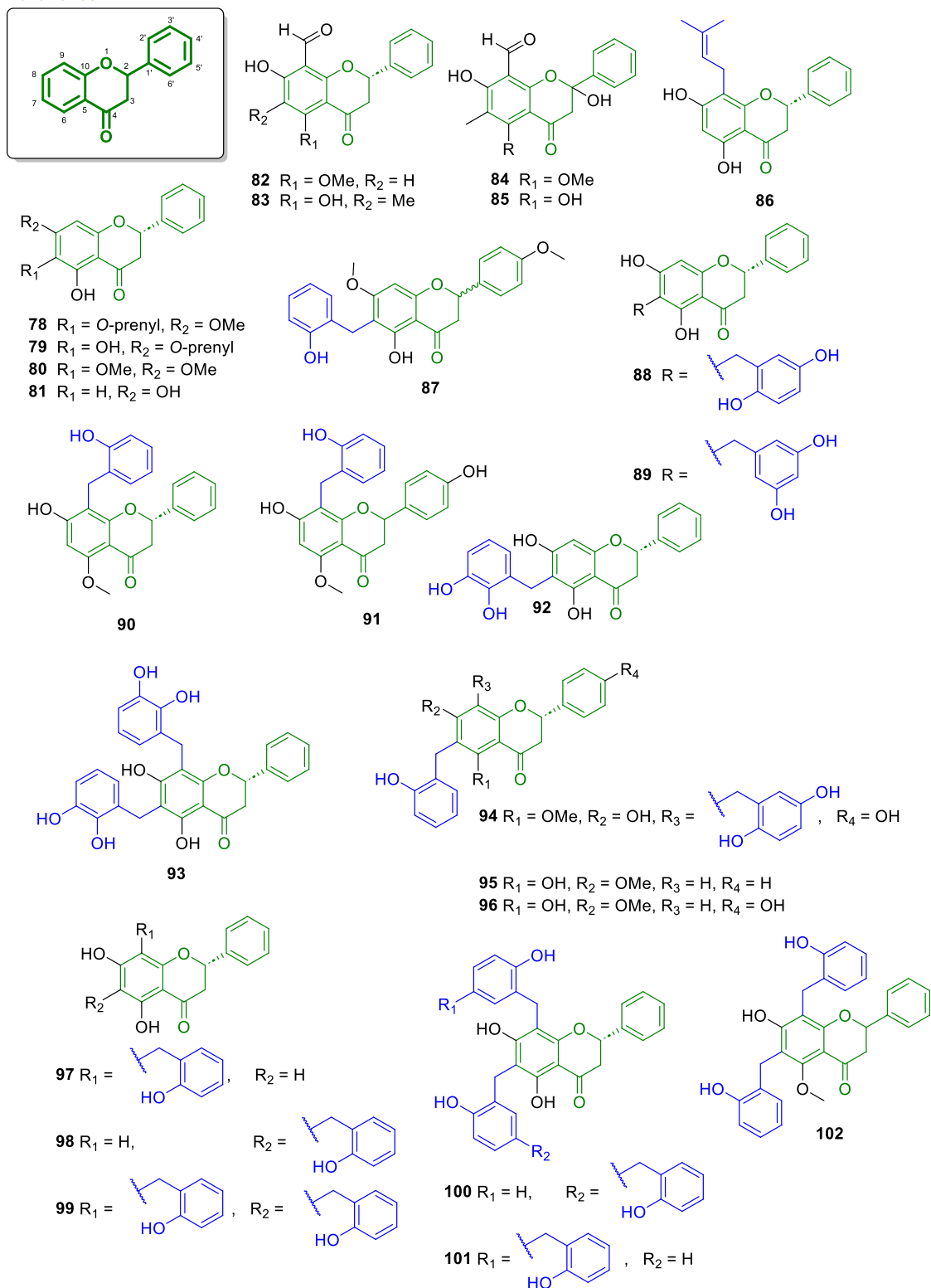
FIGURE 7 Chemical structures of flavanones isolated from Annonaceae (82–102).
