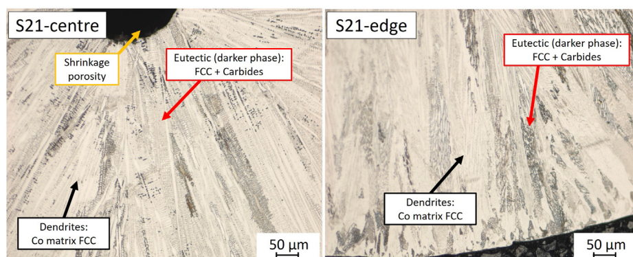
FIGURE 8 Optical microscopy of cast sample S21.
