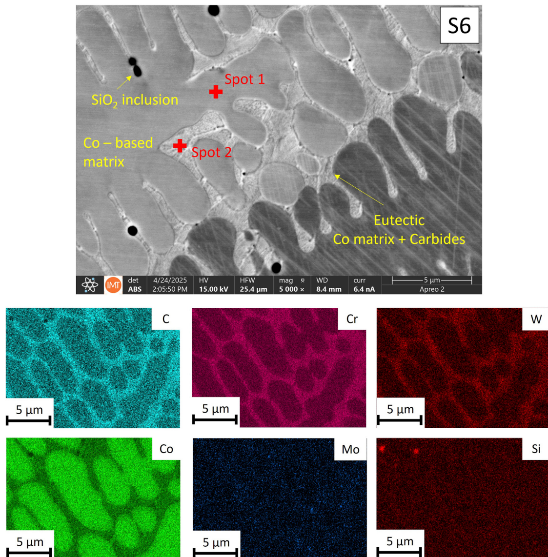
FIGURE 13 Backscattered SEM image of S6 samples and EDS elemental mapping of C, Cr, W, Co, Mo and Si.
