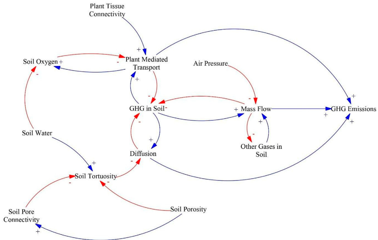
FIGURE 6 | Causal loop diagram of the main effects of water table management on greenhouse gas transport in soils. An arrow with a plus sign (blue) indicates a change in the variable affected that is in the same direction as the change in the driving variable, an arrow with a minus sign (red) indicates a change in variable affected that is in the opposite direction as the change in the driving variable.
