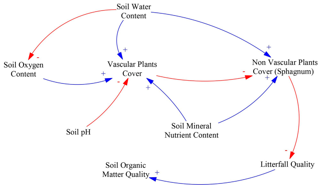
FIGURE 2 | Causal loop diagram of the main effects of water table management on litterfall quality. An arrow with a plus sign (blue) indicates a change in the variable affected that is in the same direction as the change in the driving variable, an arrow with a minus sign (red) indicates a change in variable affected that is in the opposite direction as the change in the driving variable.
