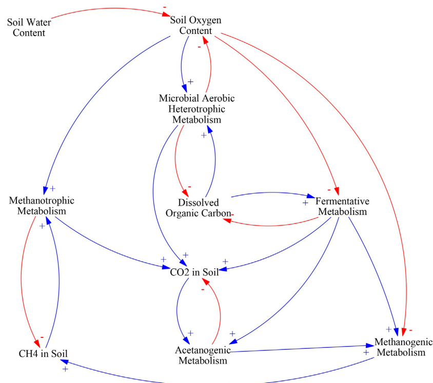
FIGURE 4 | Causal loop diagram of the main effects of water table management on carbon mineralization pathways. An arrow with a plus sign (blue) indicates a change in the variable affected that is in the same direction as the change in the driving variable, an arrow with a minus sign (red) indicates a change in variable affected that is in the opposite direction as the change in the driving variable.
