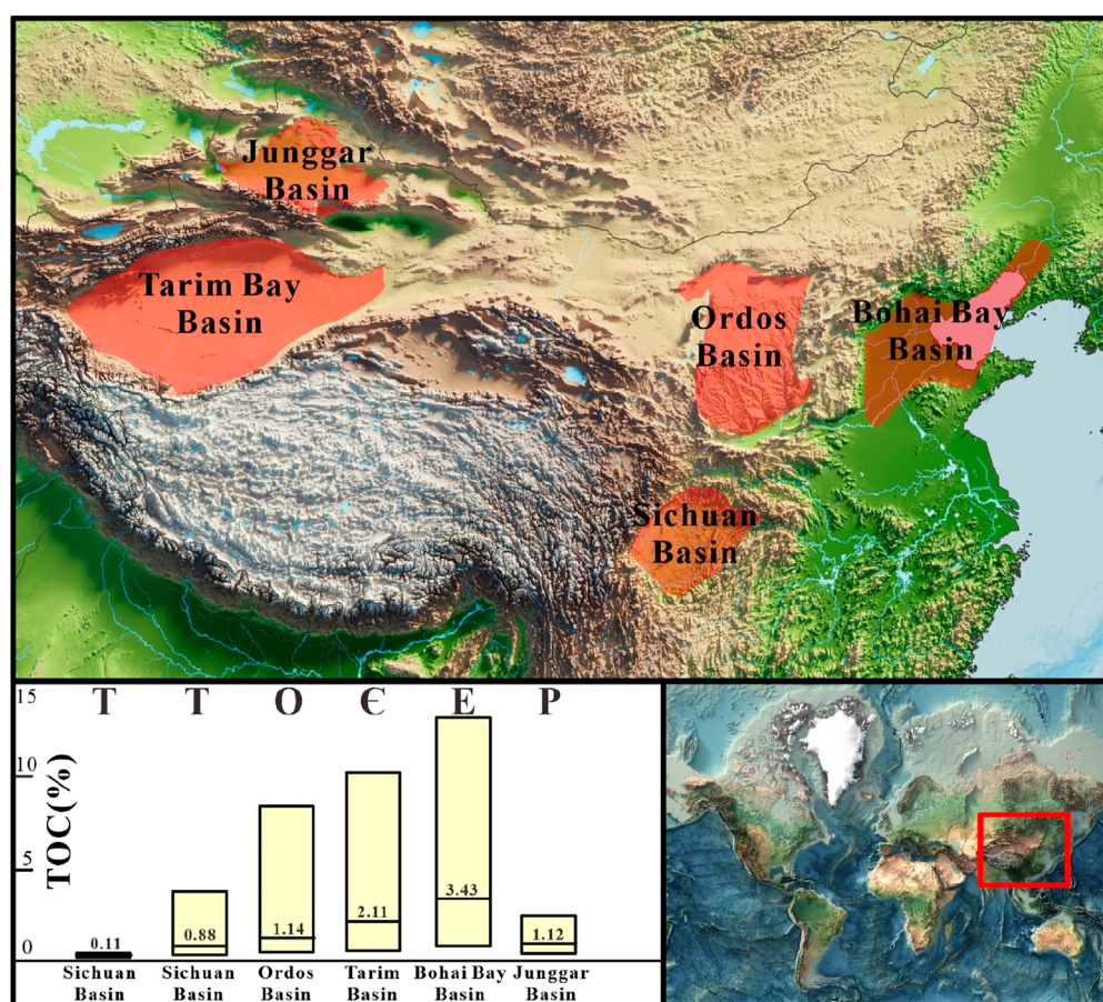
FIGURE 12 Distribution of source rocks deposited in high salinity environments in East Asia (TOC data from Tu et al., 2016 ; Duan et al., 2022 ; Guo et al., 2023 ; Zhang et al., 2023 ; Bai et al., 2024 ).
