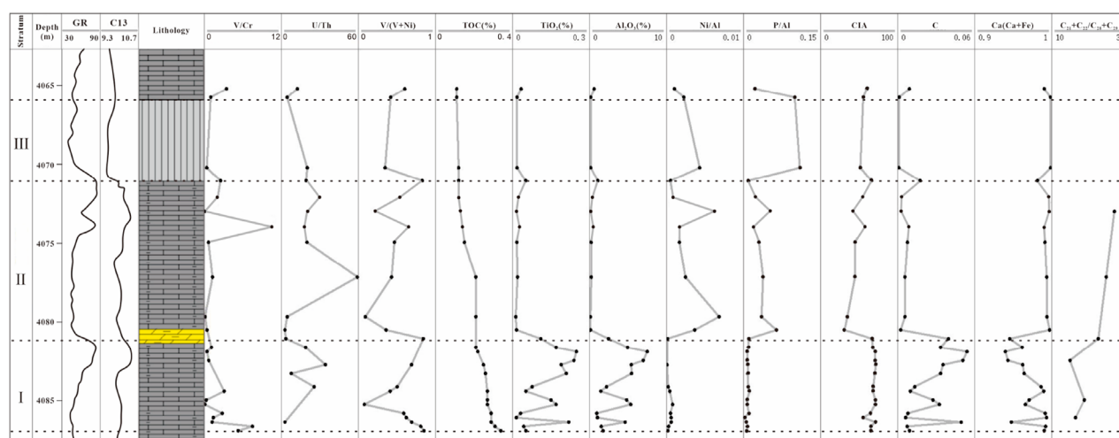
FIGURE 7 Longitudinal changes of redox, terrigenous input, paleoproductivity, CIA, C index, paleosalinity, and TOC in PY3 well.
