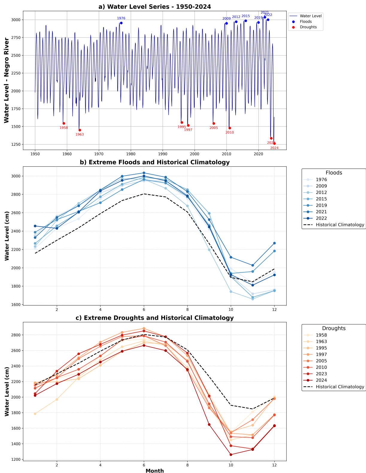
FIGURE 7 Evolution of water levels in the Rio Negro at the Manaus station between 1950 and 2024. (a) River level time series—the historical series shows the annual variation of the Negro River level, highlighting years of extreme floods (blue points) and extreme droughts (red points). (b) Extreme floods and historical climatology—the seasonal variation of the river level for extreme flood years (blue-violet lines) compared to the historical climatology (dashed black line). (c) Extreme droughts and historical climatology—the seasonal variation of the river level for extreme drought years (orange-red lines) compared to the historical climatology (dashed black line).
