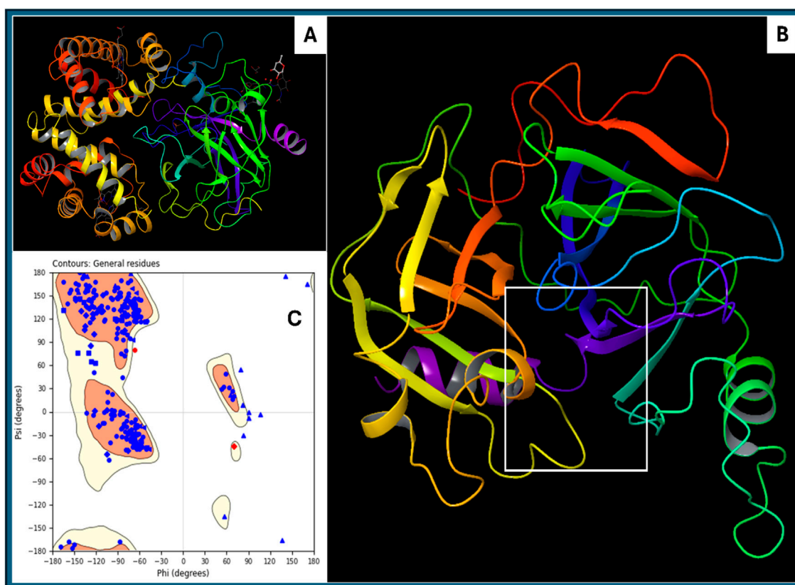
FIGURE 2 Showing the (A) downloaded haptoglobin structure in 3D, (B) prepared clean structure of haptoglobin with marked ligand binding site (white box), and (C) Ramachandran Plot for the Prepared structure of the protein.
