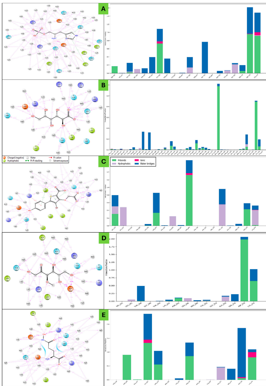
FIGURE 8 Showing the Molecular Dynamics-based Simulation Interaction Diagram (SID) and its histogram representations for haptoglobin in complex with (A) L-histidinol phosphate (DB03997), (B) L-Gluconic Acid (DB04304), (C) 4-bromo-3-(carboxymethoxy)-5-(4-hydroxyphenyl)thiophene-2-carboxylic acid (DB07197), (D) 3-O-Methylfructose (DB02438), and (E) Glutamine hydroxamate (DB02446). The legend is in different colours to differentiate the plots' bonds and residue types.
