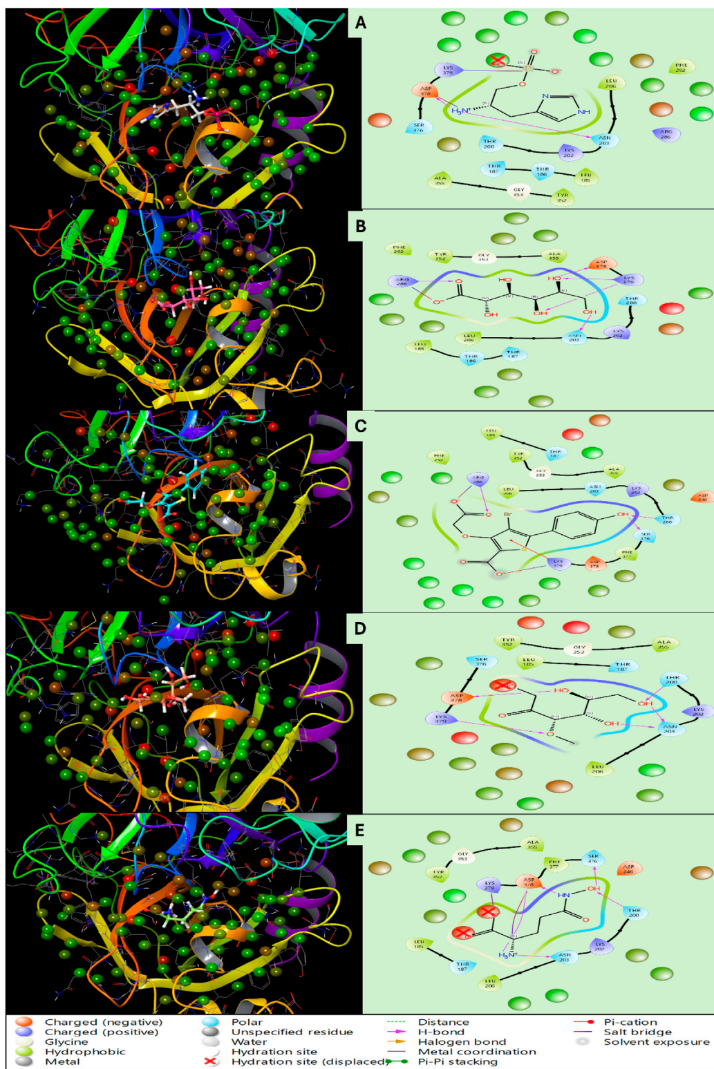
FIGURE 6 Showing the WaterMap Results in 3D and 2D Ligand Interaction Diagram for Haptoglobin in complex with (A) L-histidinol phosphate (DB03997), (B) L-Gluconic Acid (DB04304), (C) 4-bromo-3-(carboxymethoxy)-5-(4-hydroxyphenyl)thiophene-2-carboxylic acid (DB07197), (D) 3-O-Methylfructose (DB02438), and (E) Glutamine hydroxamate (DB02446) and legend is shown for various bond and residue types.
