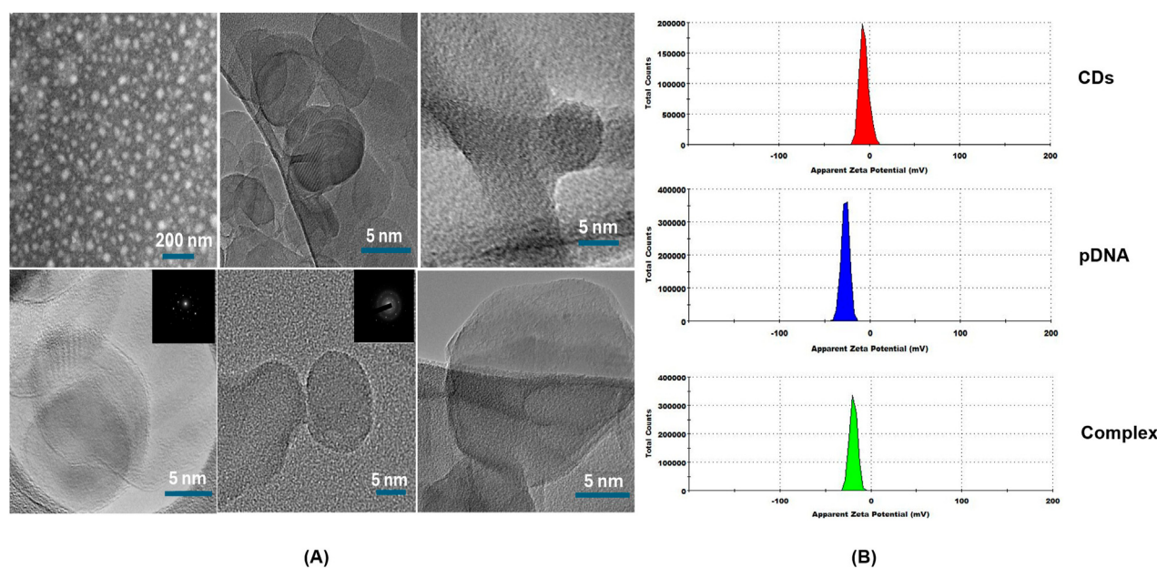
FIGURE 4 (A) High-resolution transmission electron microscopy (HRTEM) and Dark-field scanning transmission electron microscopy (STEM) images of carbon dots. (B) Zeta-potential of carbon dots (CDs), plasmid DNA (pDNA) and the complex of carbon dots and plasmid DNA (Complex).
