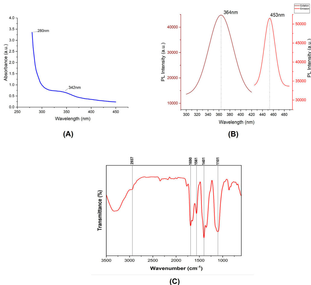
FIGURE 3 (A) Absorption spectrum of the synthesized CDs, displaying prominent peaks at 280 nm and 342 nm. (B) Fluorescence spectra of the synthesized CDs, including excitation and emission spectra. (C) FTIR spectrum illustrating the functional groups present in the Citric acid/ \beta -alanine-derived carbon dots.
